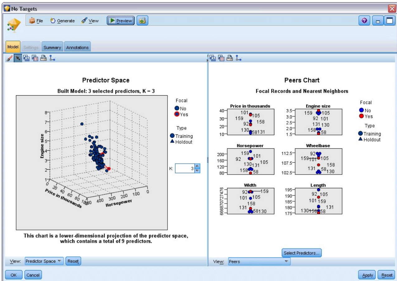
Figura 391. La ventana Model Viewer
